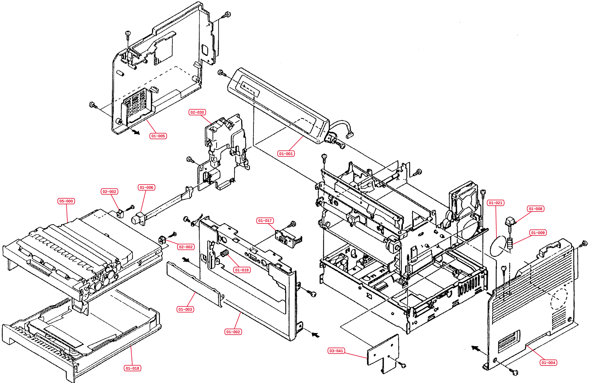
Fig.1 – Covers
