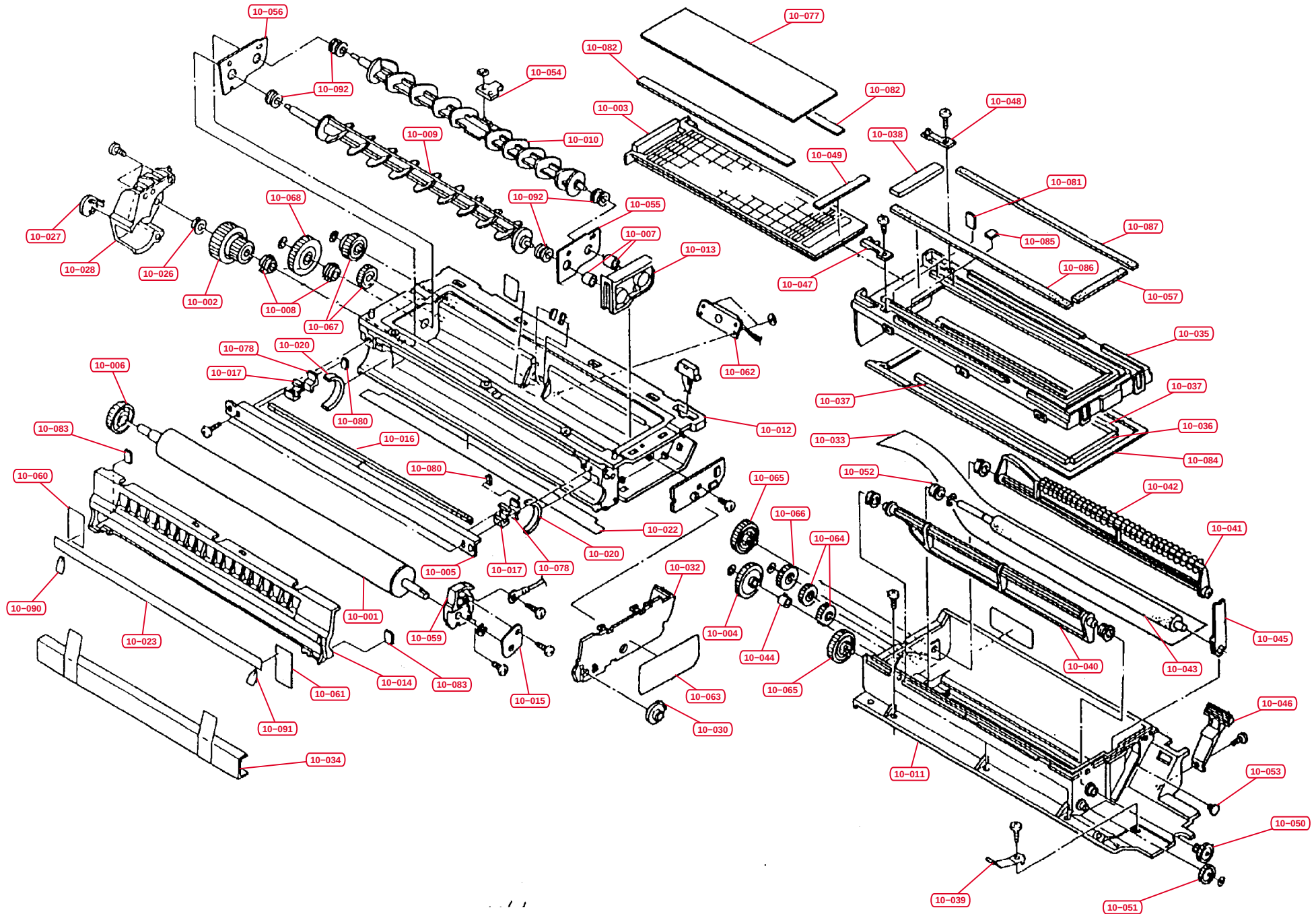
Fig.10 - Developer Unit
