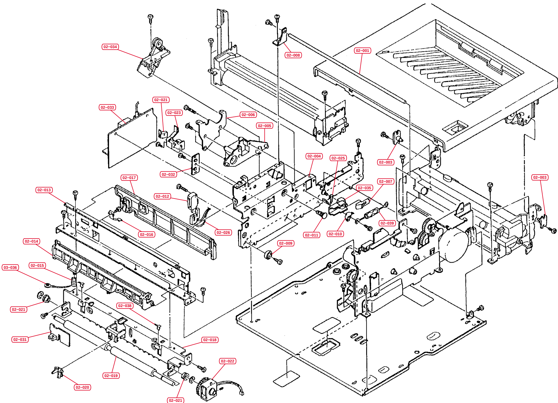
Fig.2 – Frame Unit
