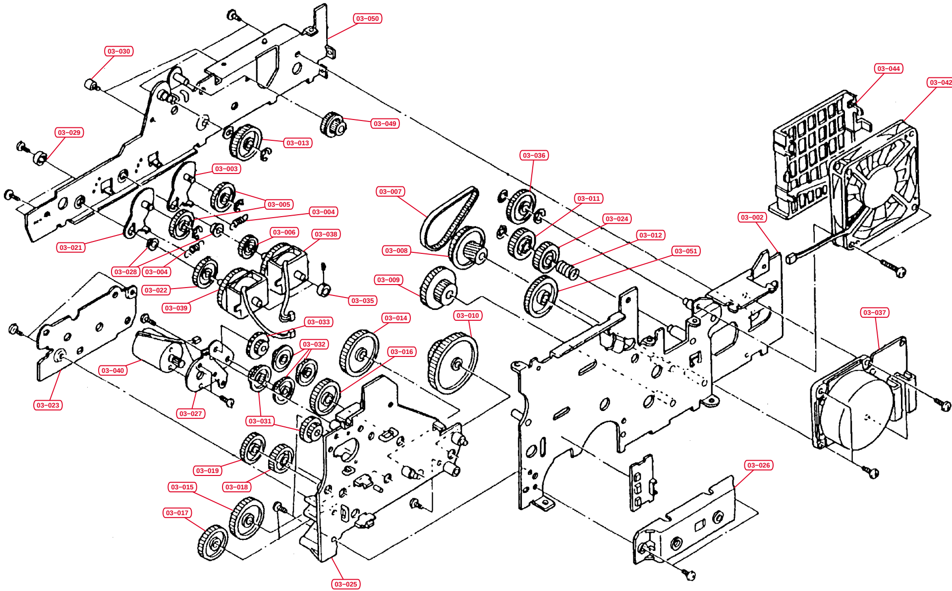
Fig.3 – Drive Frame Unit
